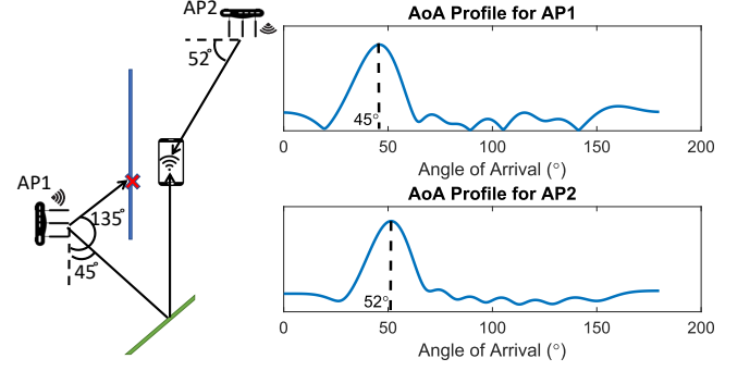
Figure 2: Traditional Localization Approach: WiFi signals transmitted by a smartphone are measured at multi-antenna access points. The access points infer angle of arrival information. However, in the absence of a direct path, this information is erroneous and can lead to large errors (3 to 5m).
