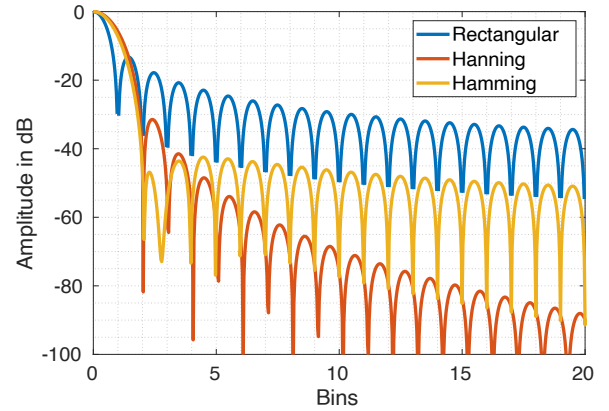
Figure 5: Frequency response of common window functions
