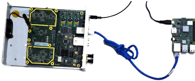
Figure 13: SparSDR reconstructs 100-MHz captures in near real time on a Raspberry Pi.
