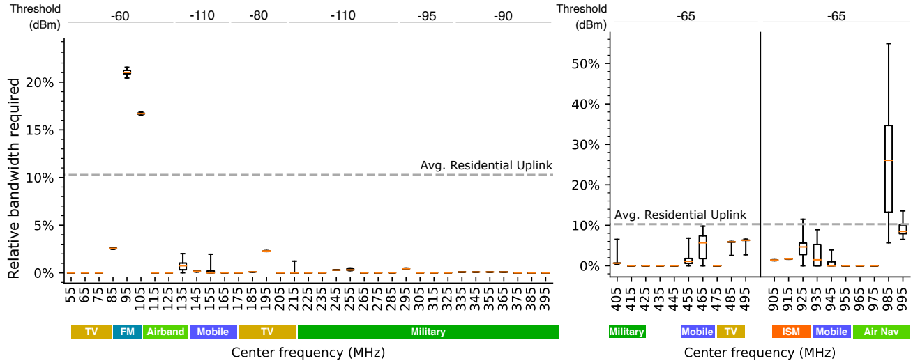
Figure 16: The distribution of SparSDR's backhaul for capturing transmissions in 10-MHz bands from 50 MHz to 1 GHz. Bandwidth is plotted relative to the 320 Mbps needed by a standard 10-MHz SDR. We also indicate the capacity of a typical residential-class Internet uplink.
