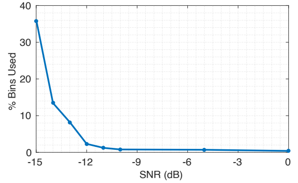
Figure 11: Average fraction of STFT bins that were above the threshold to achieve BER of less than 10^{-5} for different SNR values. Evaluated signal is IEEE 802.15.4 (ZigBee) PHY with 2 MHz of bandwidth.
